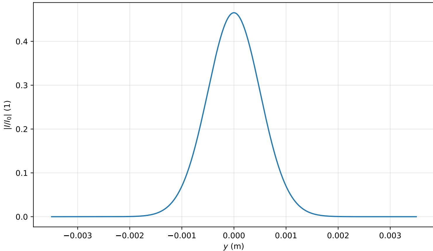
Intensity profile I(x = 0, y, z = 2.309)/I_0 , P_{in}=0.1P_{cr} , artificial time
